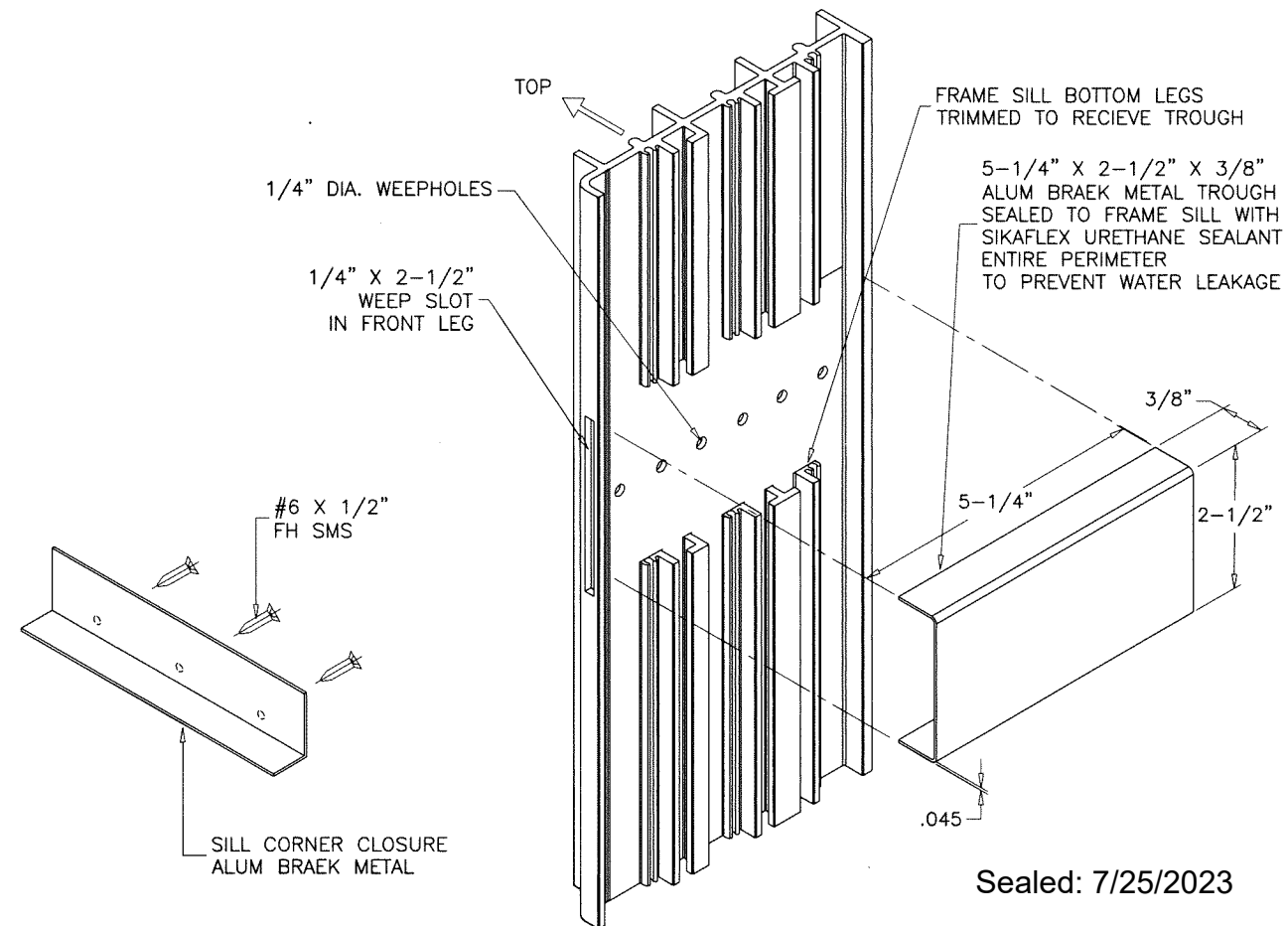
FRAME SILL BOTTOM VIEW
