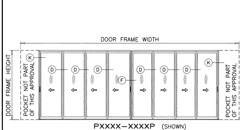
APPROVED CONFIGURATIONS POCKETED DOORS FIVE (5) TRACKS
